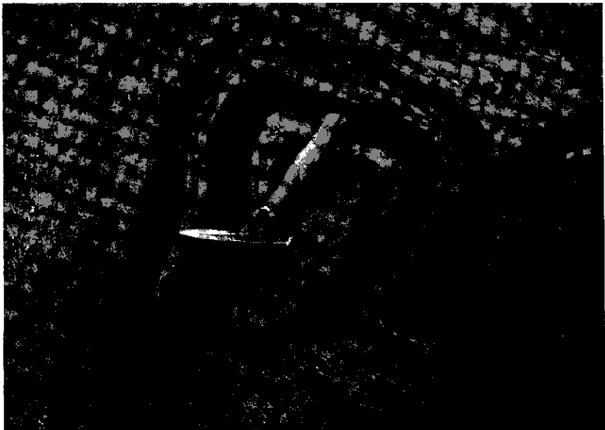
Fig. 2. Fold in banded gneiss, cut off by recrystallization.
