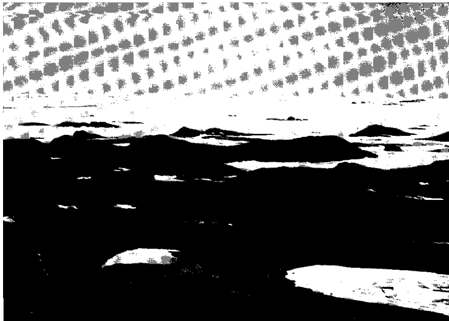
Fig. 1. Raised beach and strandline, Chapman Ridge.
