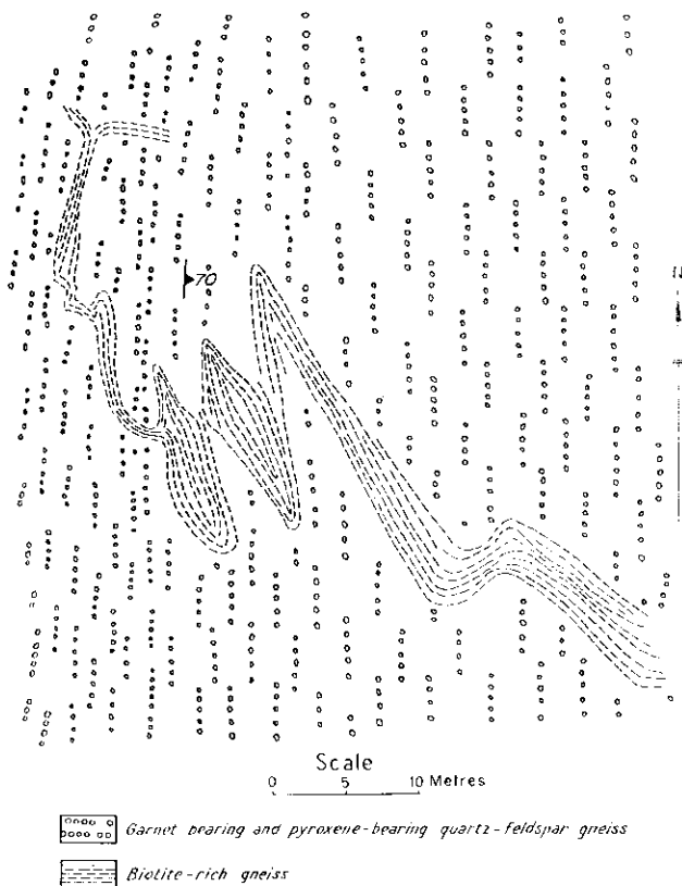
Figure 3. Sketch map of biotite-rich band transgressing foliation, Tschuffert Peak, Mac.Robertson Land, Antarctica.
