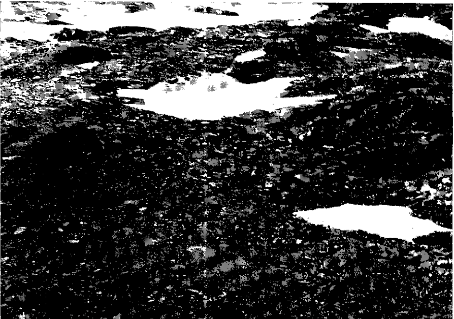
Fig. 2. Stone circles on Kemp Peak.
