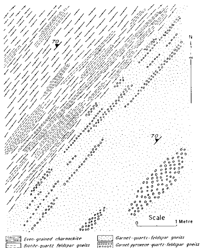
Figure 2. Diagrammatic sketch map of contact between even-grained charnockite and garnet-quartz-feldspar gneiss near Ufs Island, Mac.Robertson Land, Antarctica.
