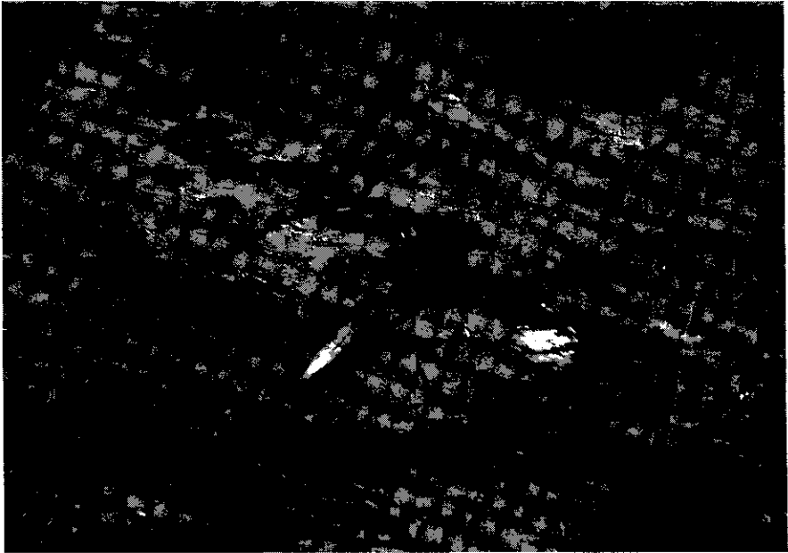
Fig. 1. Ptygmatic-like fold in banded gneiss.
